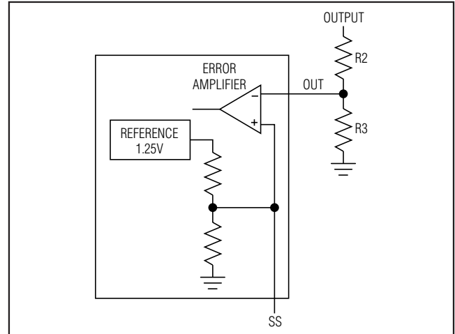
Figure 6. Adjustable Output Voltage
