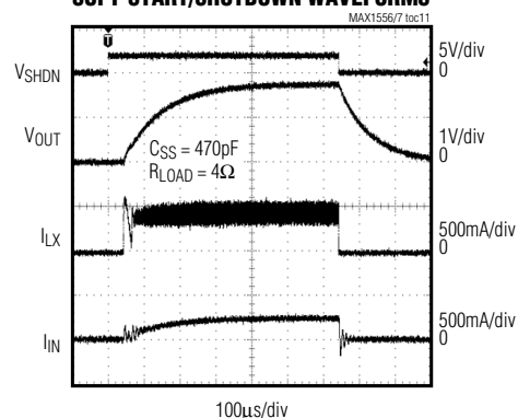
SOFT-START/SHUTDOWN WAVEFORMS
